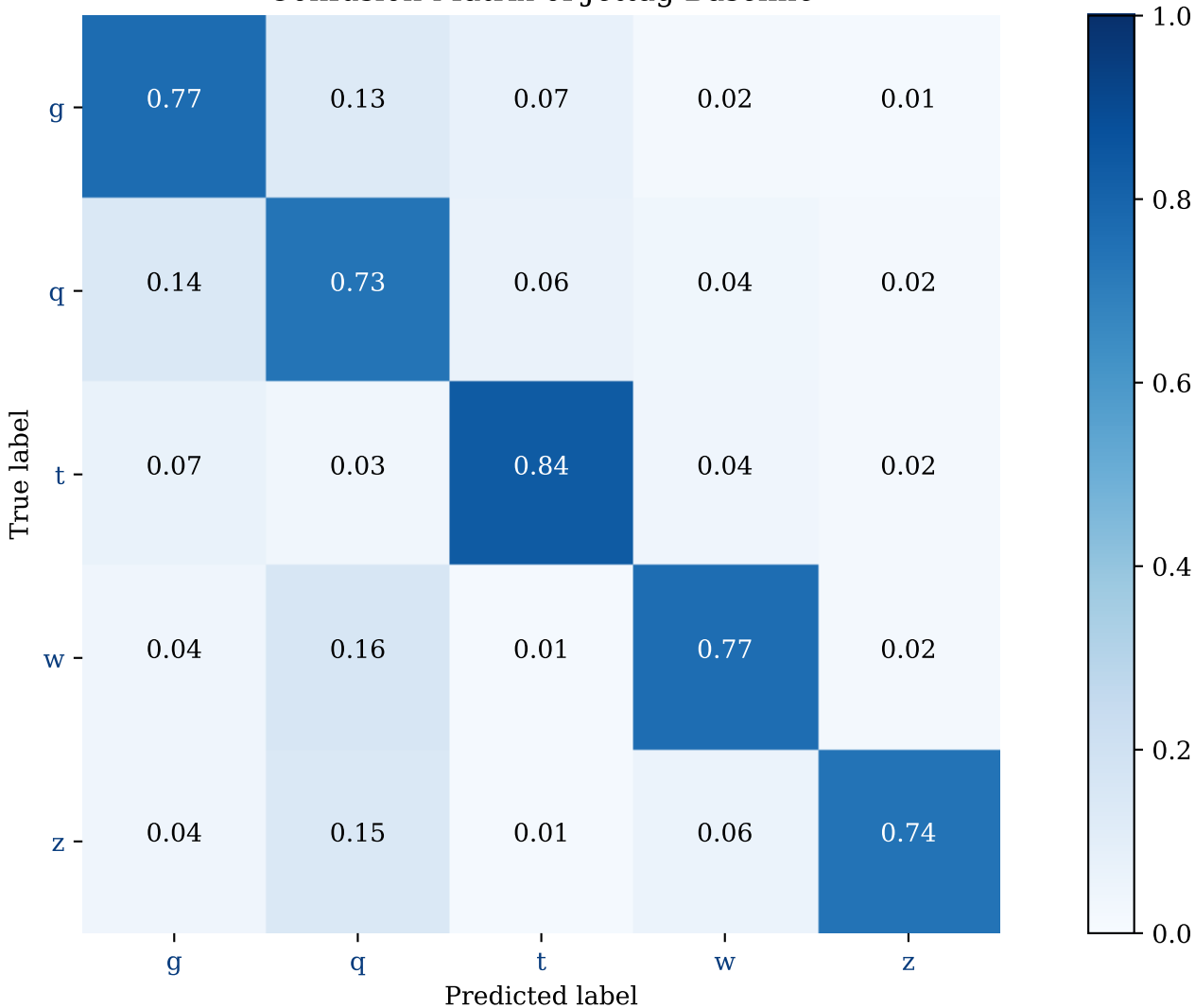
Confusion Matrix of Jettag Baseline
